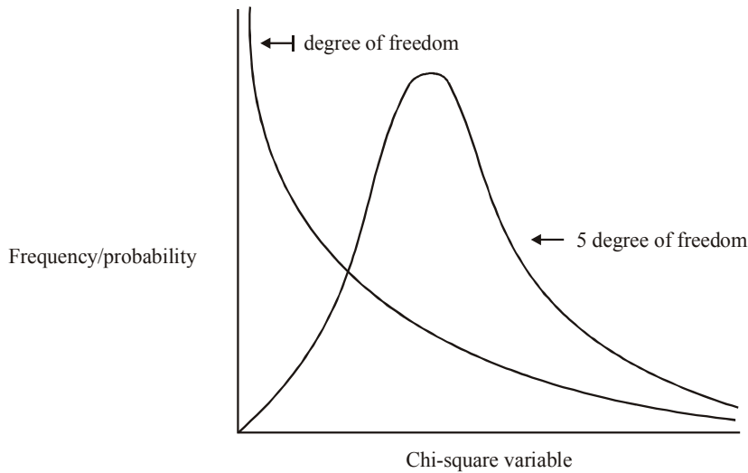
Fig. 12.3 Chi-square Distribution
